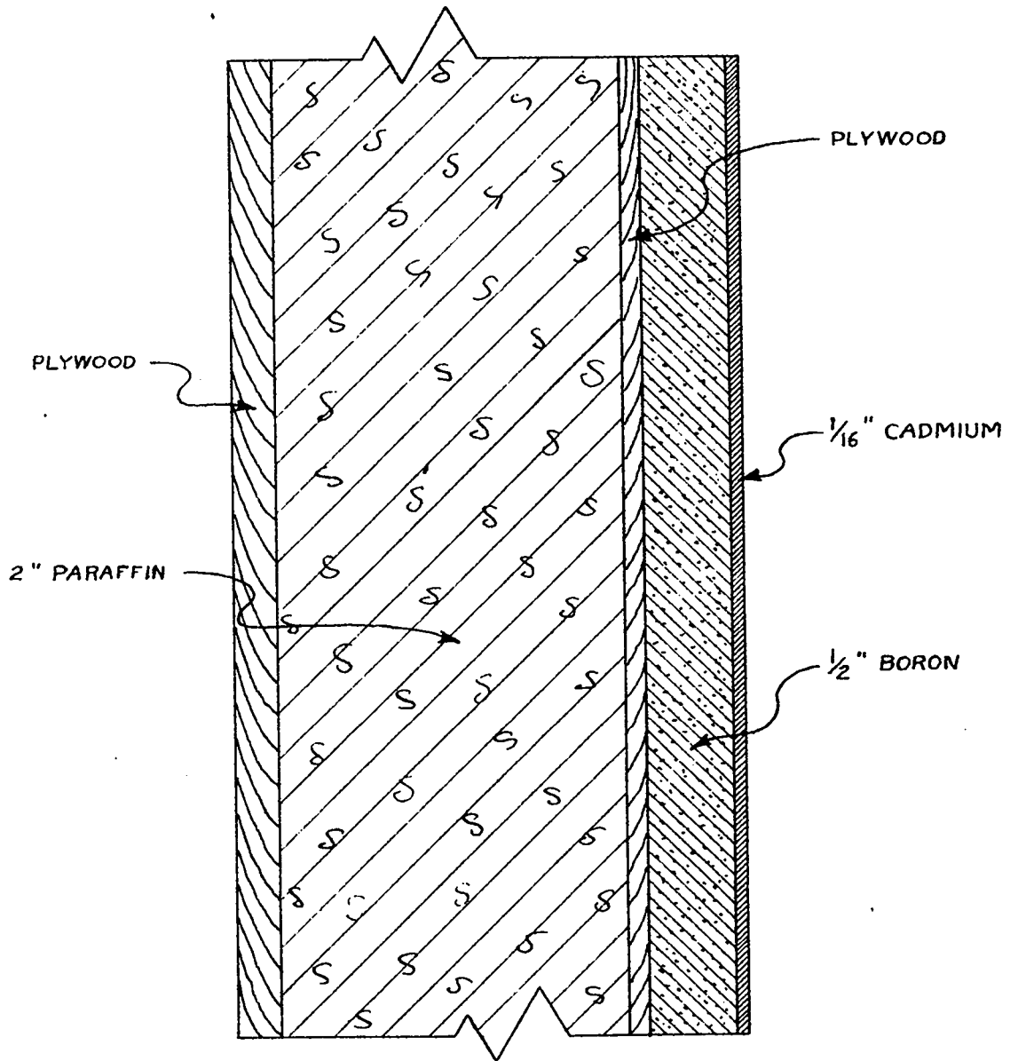
WALL CROSS-SECTION OF PARAFFIN-BORON-CADMIUM "ICE BOX"
